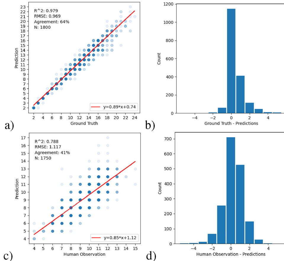
FIGURE 7 Scatter plots (a,c) and histograms (b,d) showing the prediction performance of our method. Comparison to 1800 images of unseen synthetic data (a,b) and 1750 real and manually annotated sorghum plants from Miao et al. (2021).
